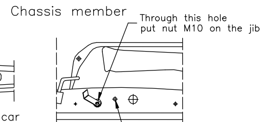
Fig. 2 Chassis member
