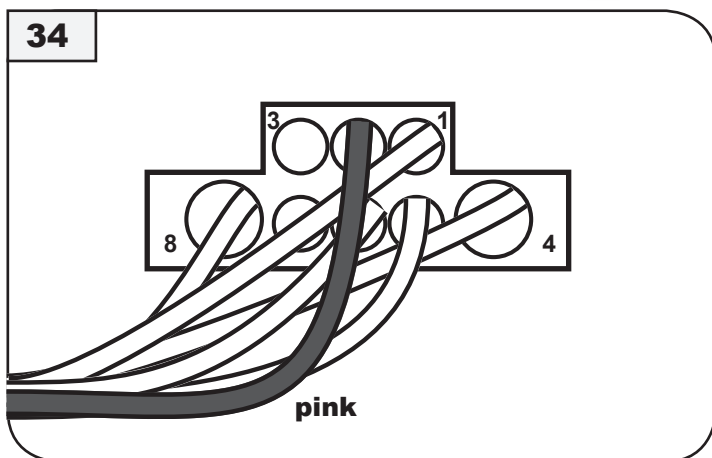
E-Satz Stecker (pink pin 2) e-kit socket (pink pin 2)
